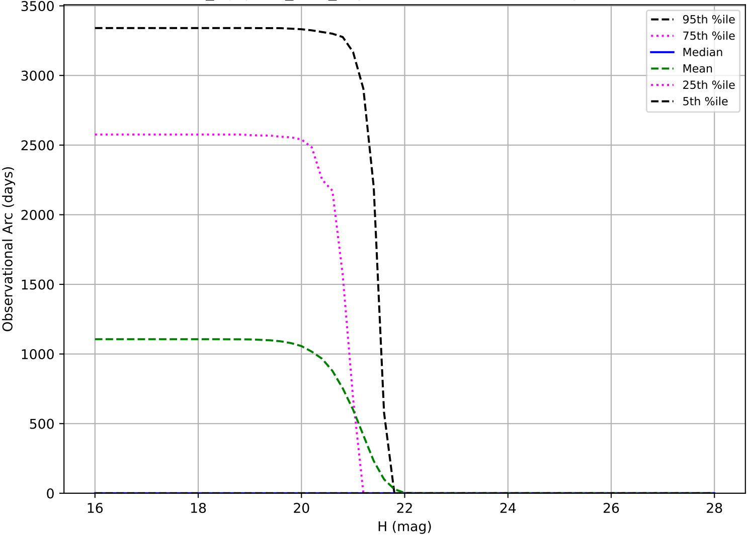
noroll_mjdp365_v3.4_10yrs: Observational Arc Length Vatira
