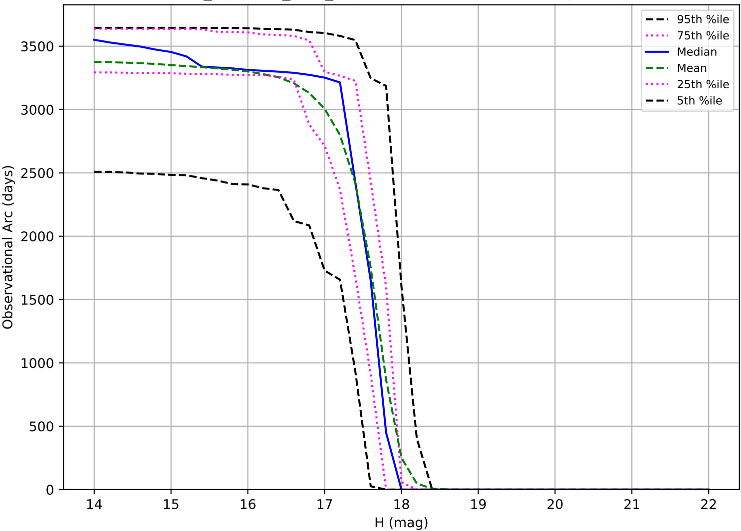
noroll_mjdp365_v3.4_10yrs: Observational Arc Length Trojan
