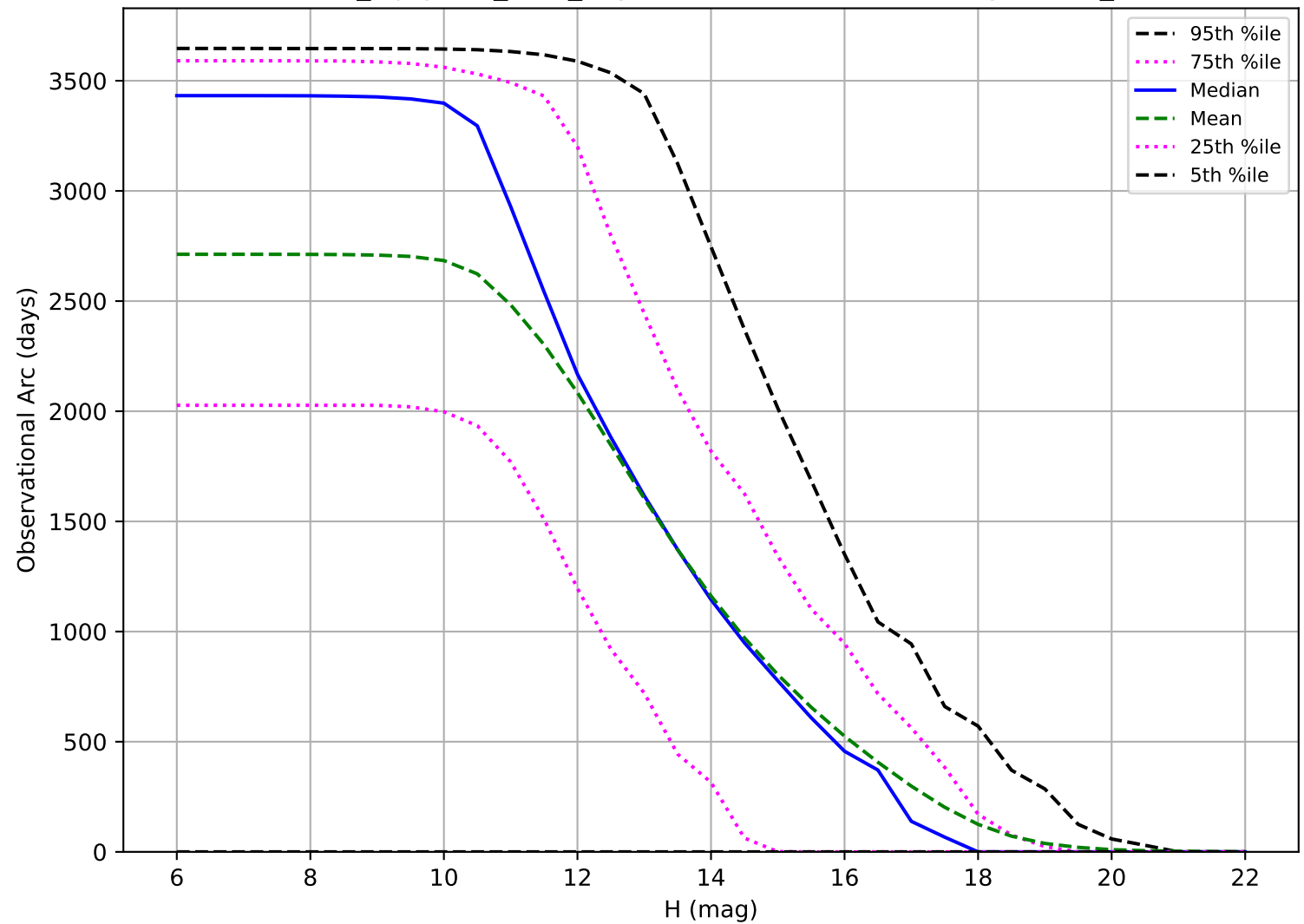
noroll_mjdp365_v3.4_10yrs: Observational Arc Length OCC_r5
