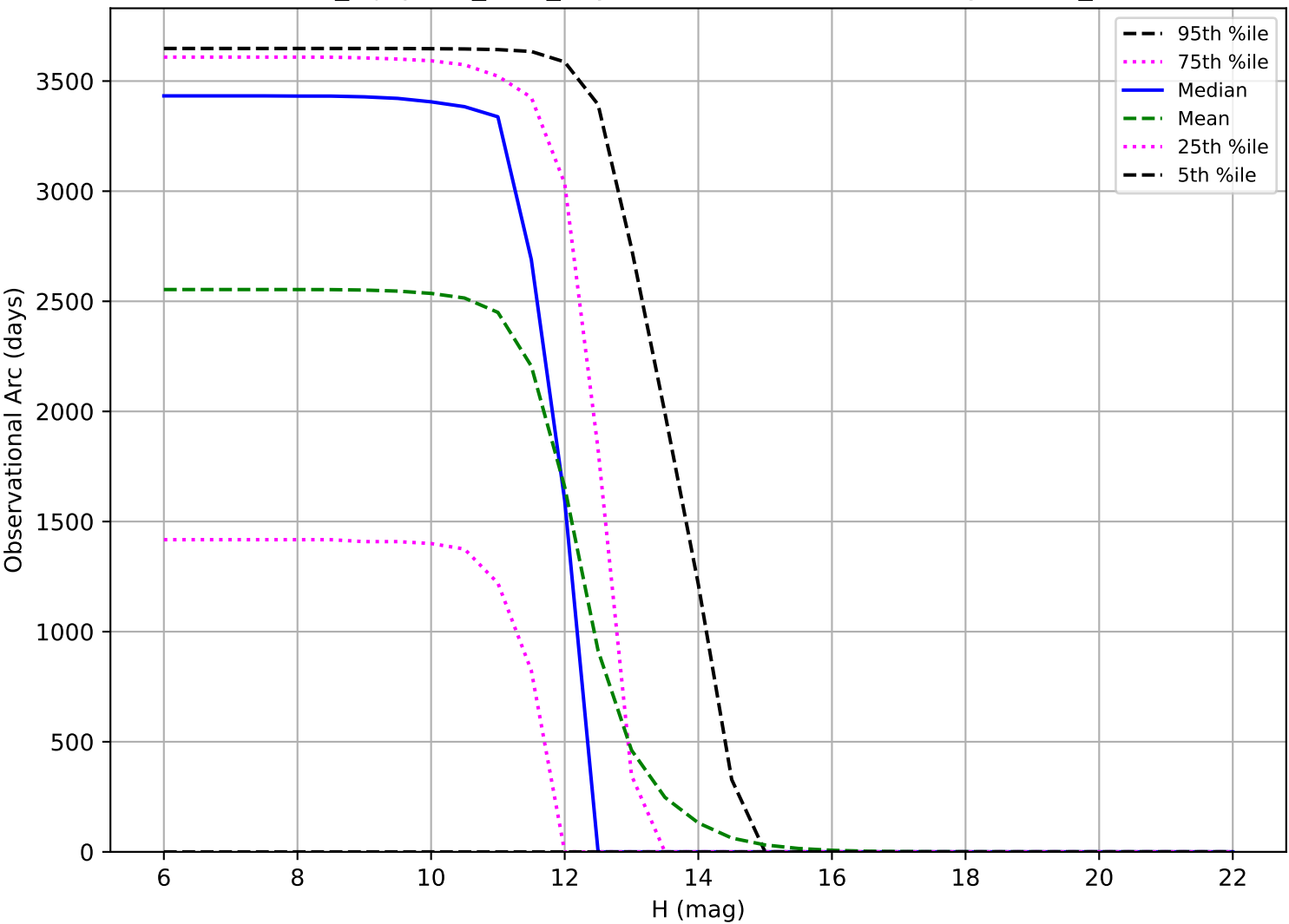
noroll_mjdp365_v3.4_10yrs: Observational Arc Length OCC_r20
