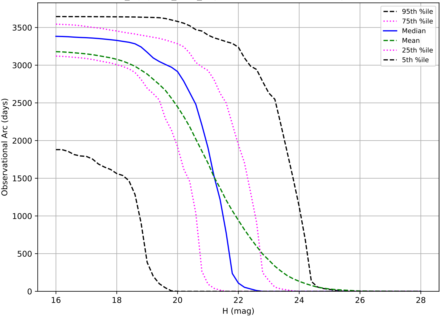
noroll_mjdp365_v3.4_10yrs: Observational Arc Length NEO
