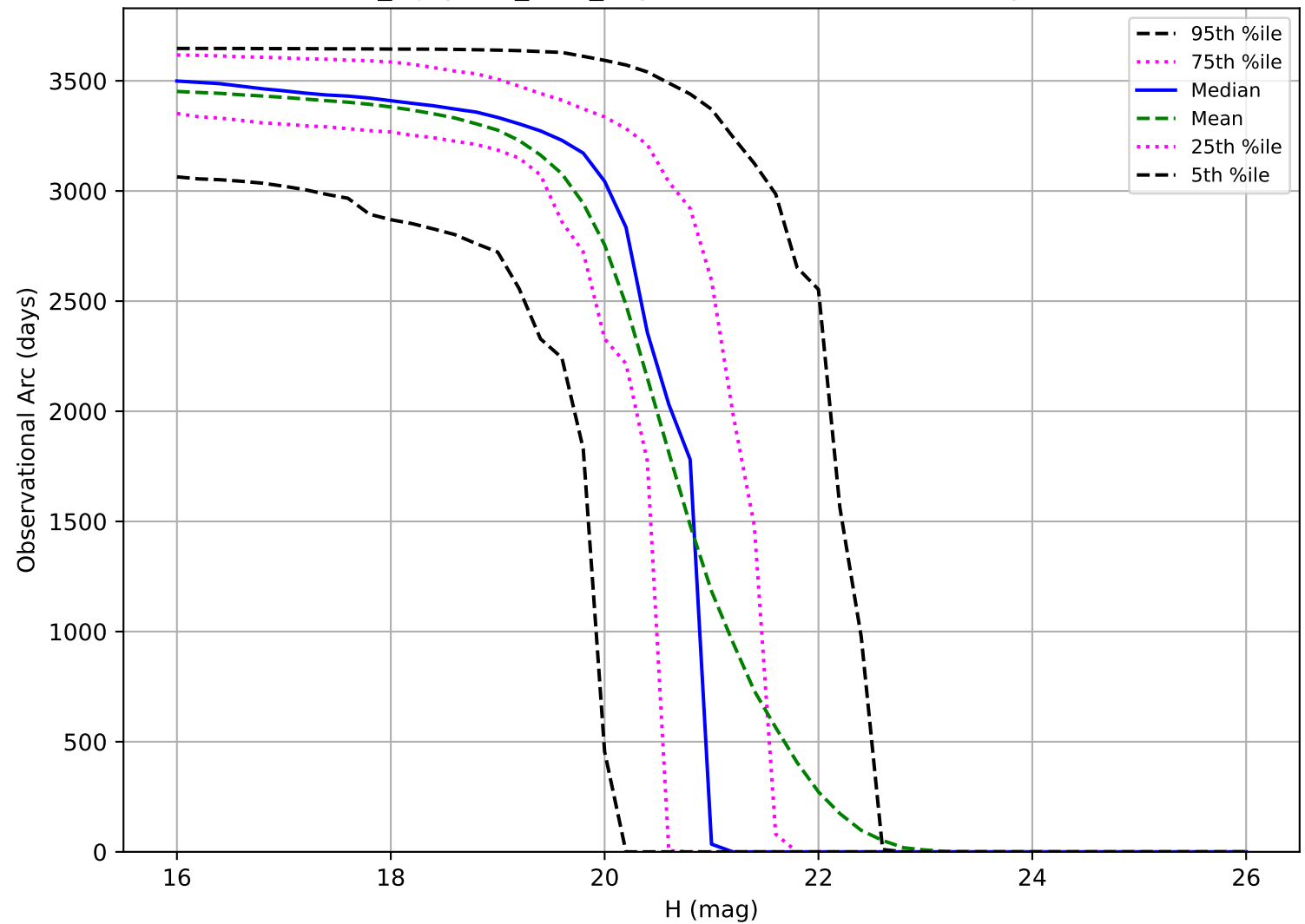
noroll_mjdp365_v3.4_10yrs: Observational Arc Length MBA
