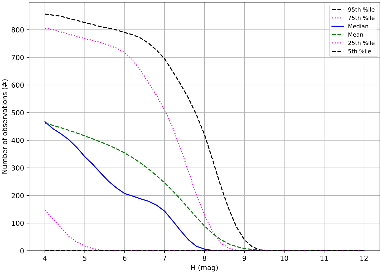
noroll_mjdp365_v3.4_10yrs: Number of observations TNO
