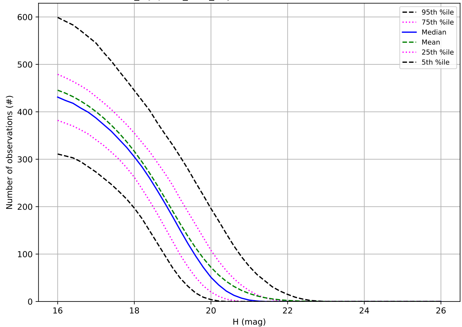
noroll_mjdp365_v3.4_10yrs: Number of observations MBA
