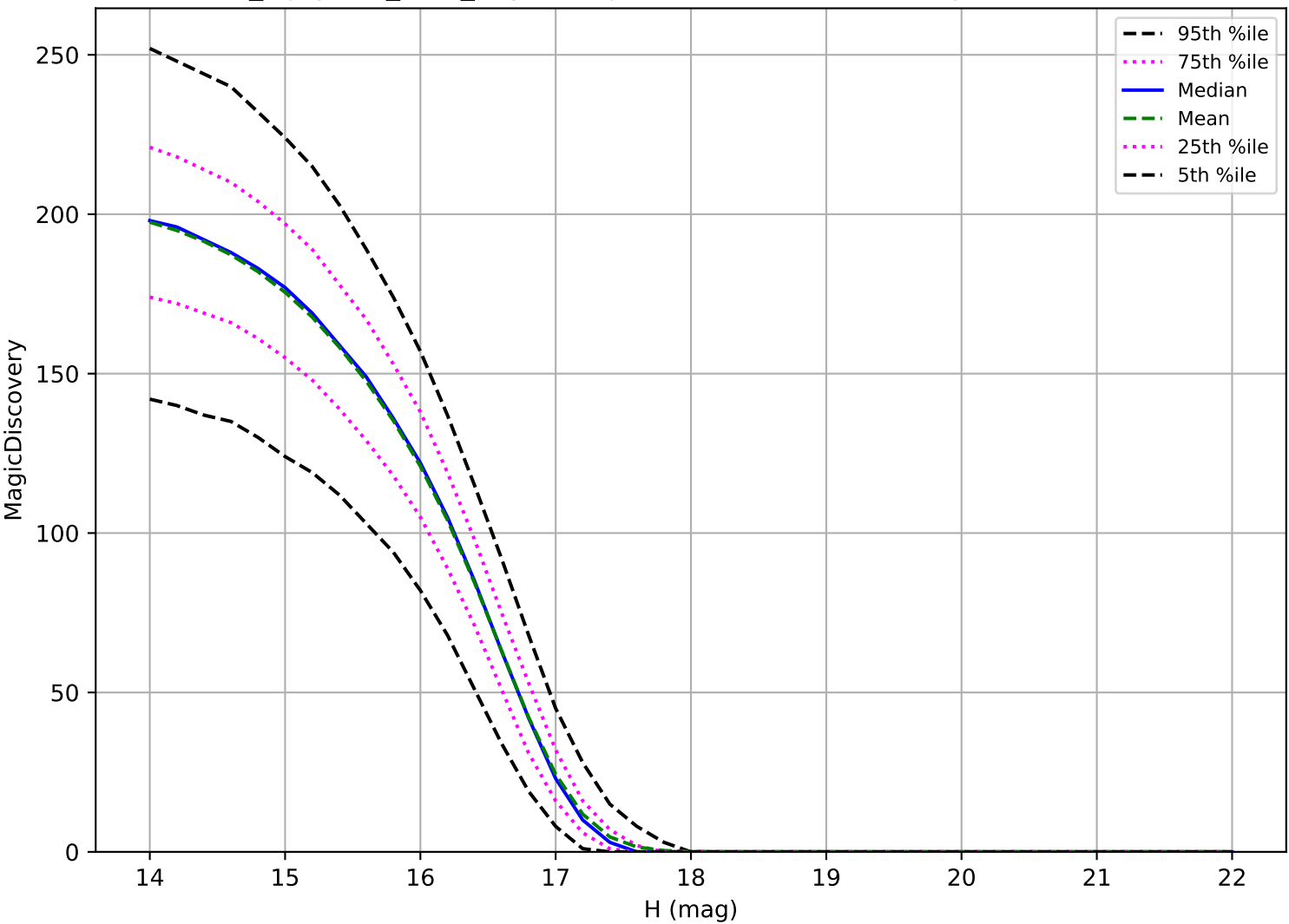
noroll_mjdp365_v3.4_10yrs: Trojan 6 detections in 60 nights detection loss
