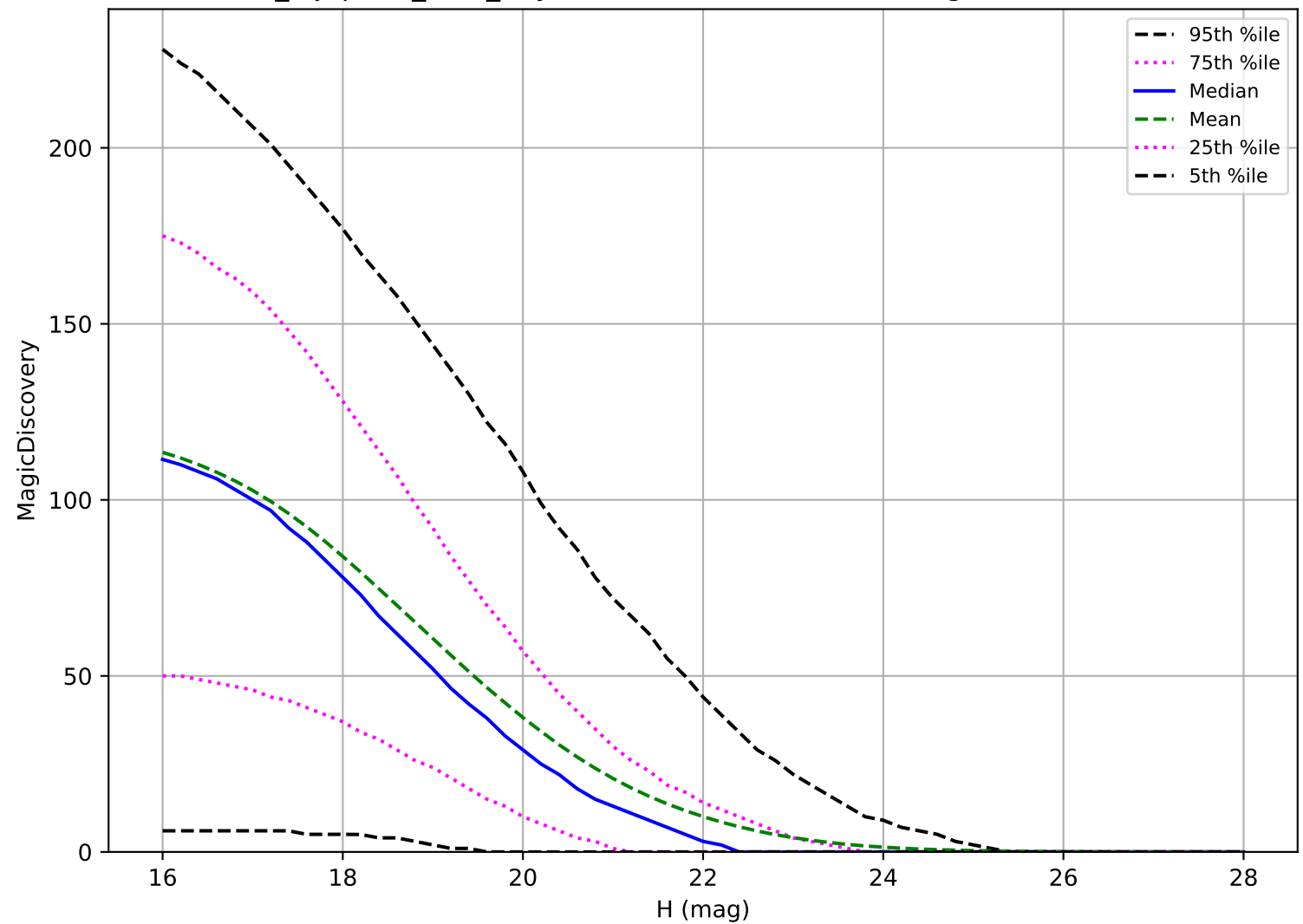
noroll_mjdp365_v3.4_10yrs: PHA 6 detections in 60 nights detection loss
