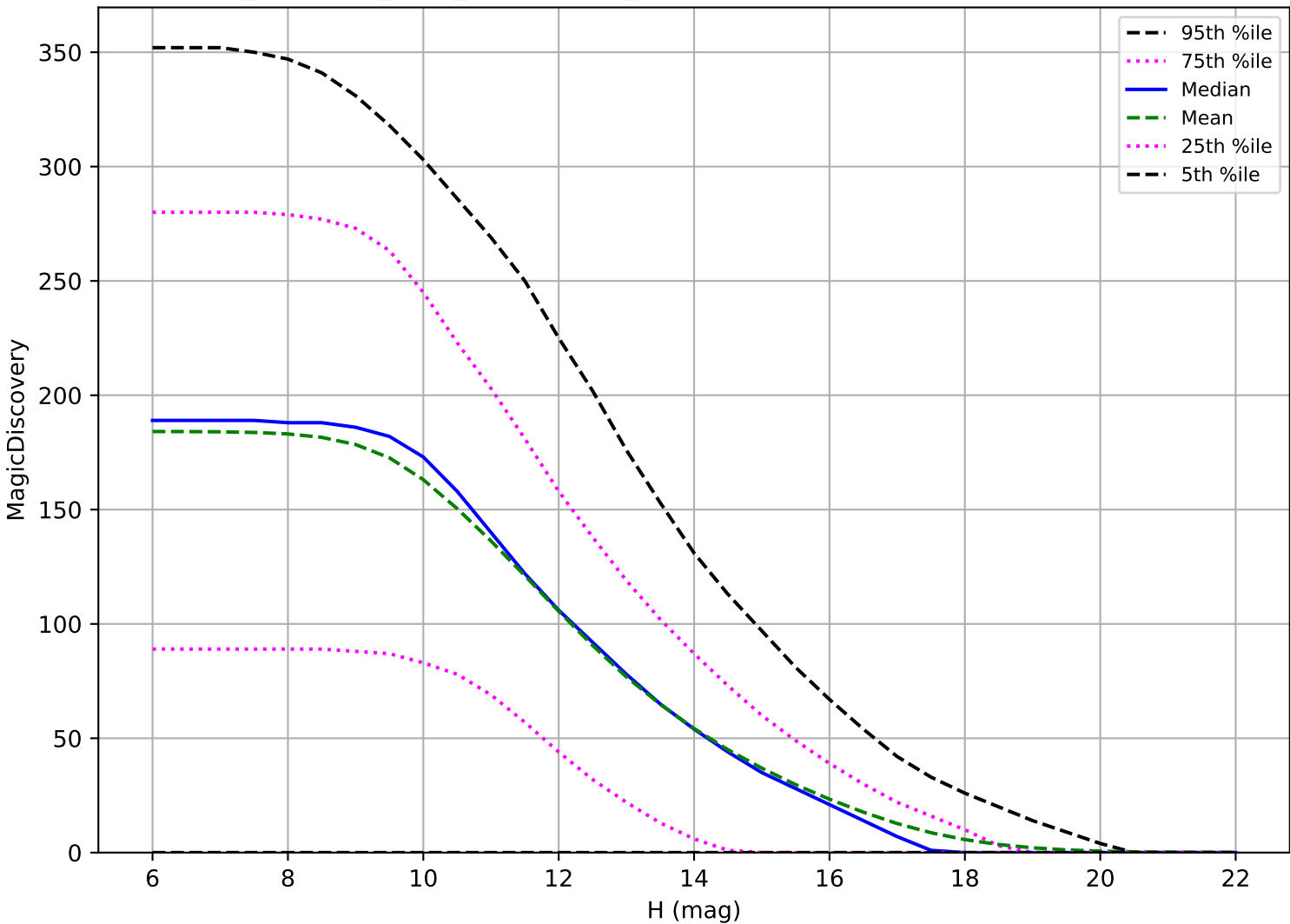
noroll_mjdp365_v3.4_10yrs: OCC_r5 6 detections in 60 nights detection loss
