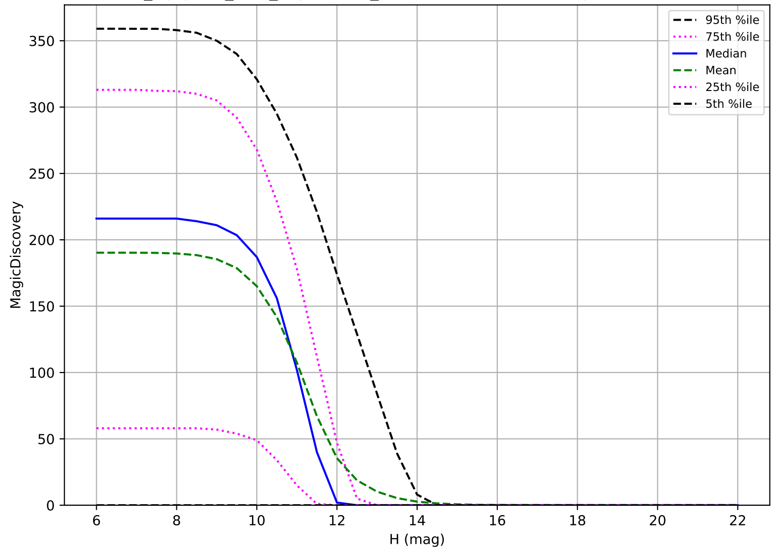
noroll_mjdp365_v3.4_10yrs: OCC_r20 6 detections in 60 nights detection loss
