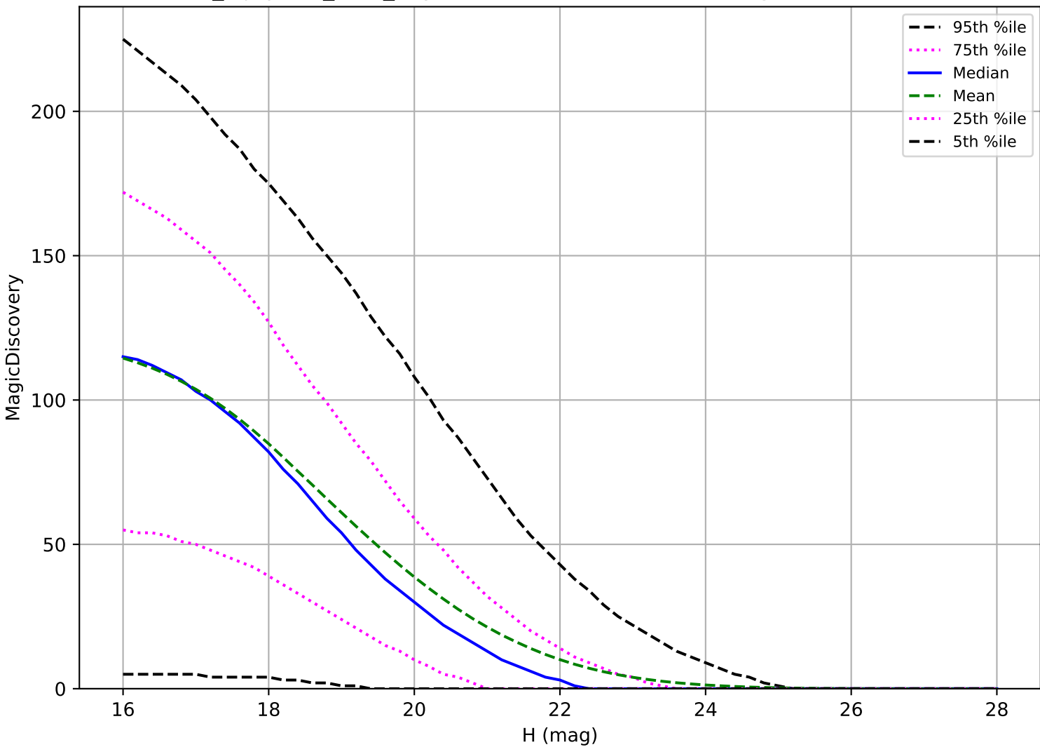
noroll_mjdp365_v3.4_10yrs: NEO 6 detections in 60 nights detection loss
