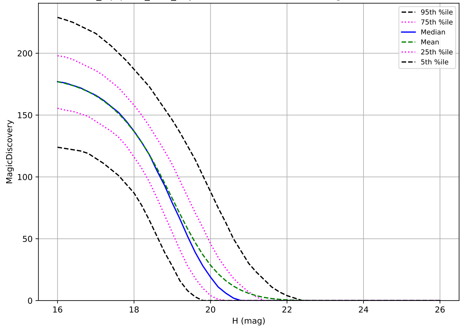
noroll_mjdp365_v3.4_10yrs: MBA 6 detections in 60 nights detection loss
