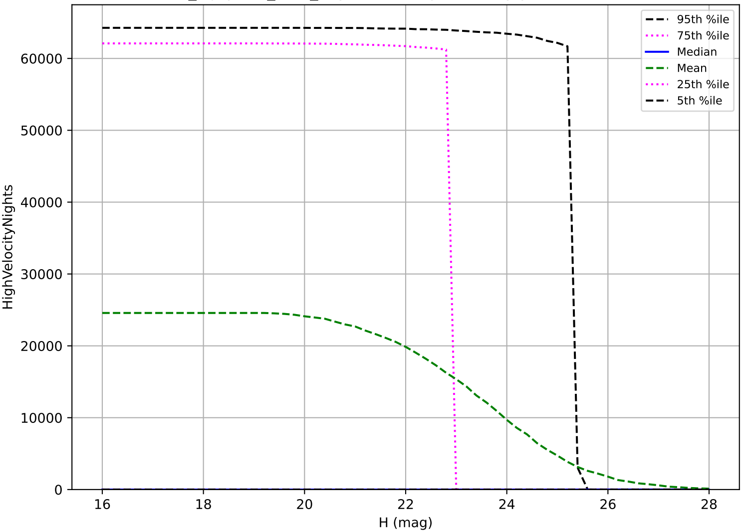
noroll_mjdp365_v3.4_10yrs: PHA High velocity pair detection loss
