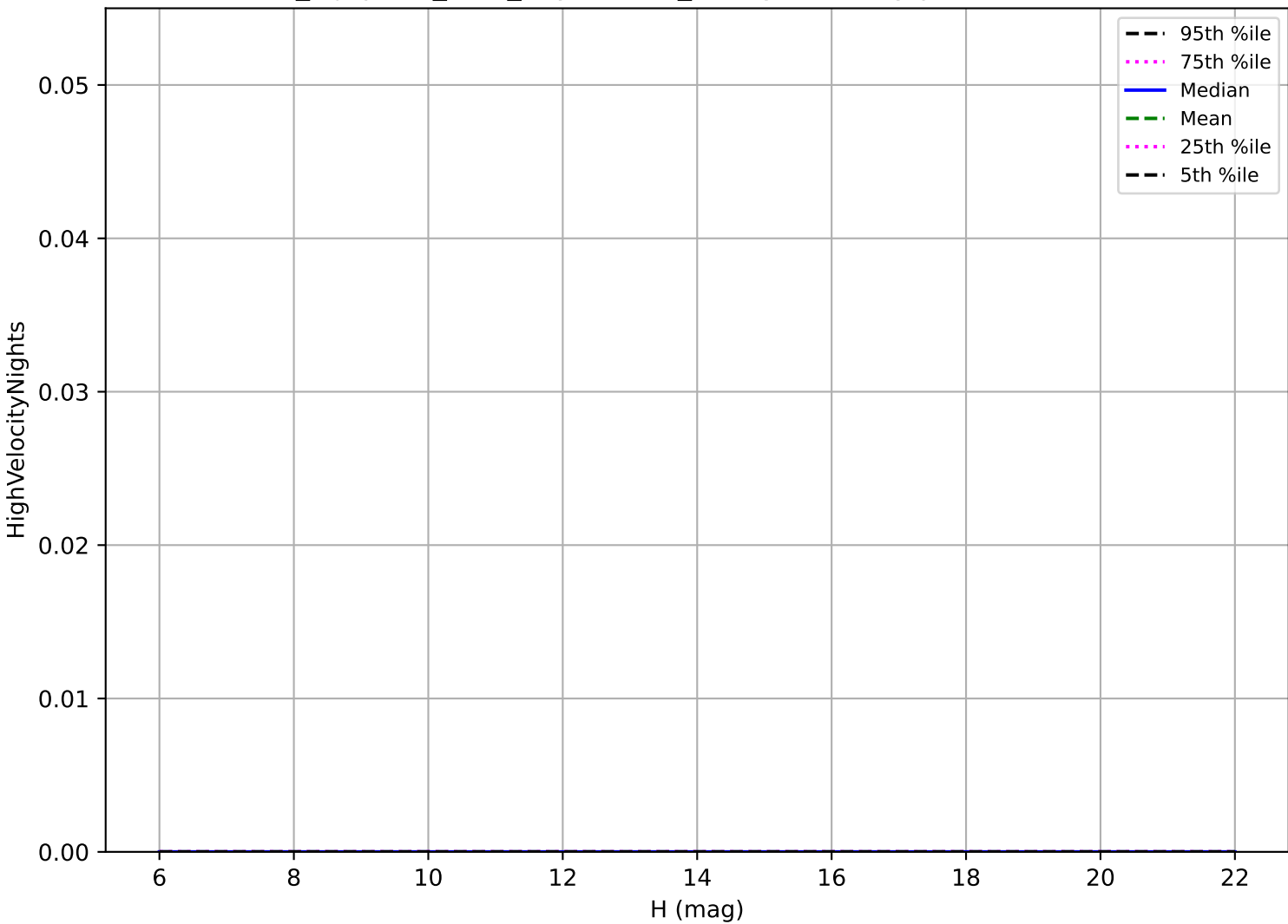
noroll_mjdp365_v3.4_10yrs: OCC_r5 High velocity pair detection loss
