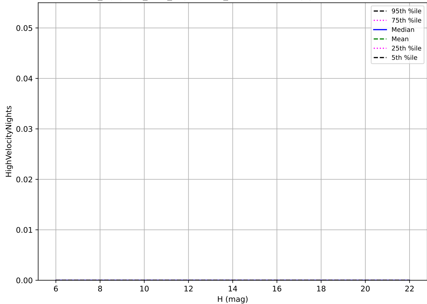
noroll_mjdp365_v3.4_10yrs: OCC_r20 High velocity pair detection loss
