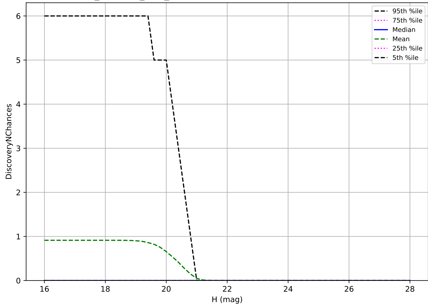
noroll_mjdp365_v3.4_10yrs: Vatira 3 pairs in 15 nights detection loss
