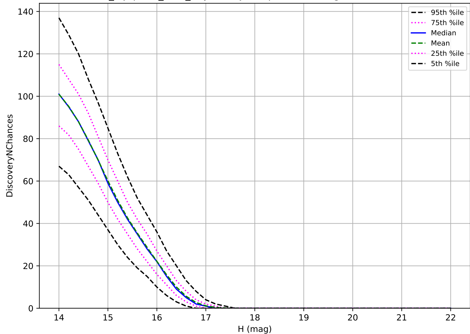
noroll_mjdp365_v3.4_10yrs: Trojan 3 pairs in 15 nights detection loss
