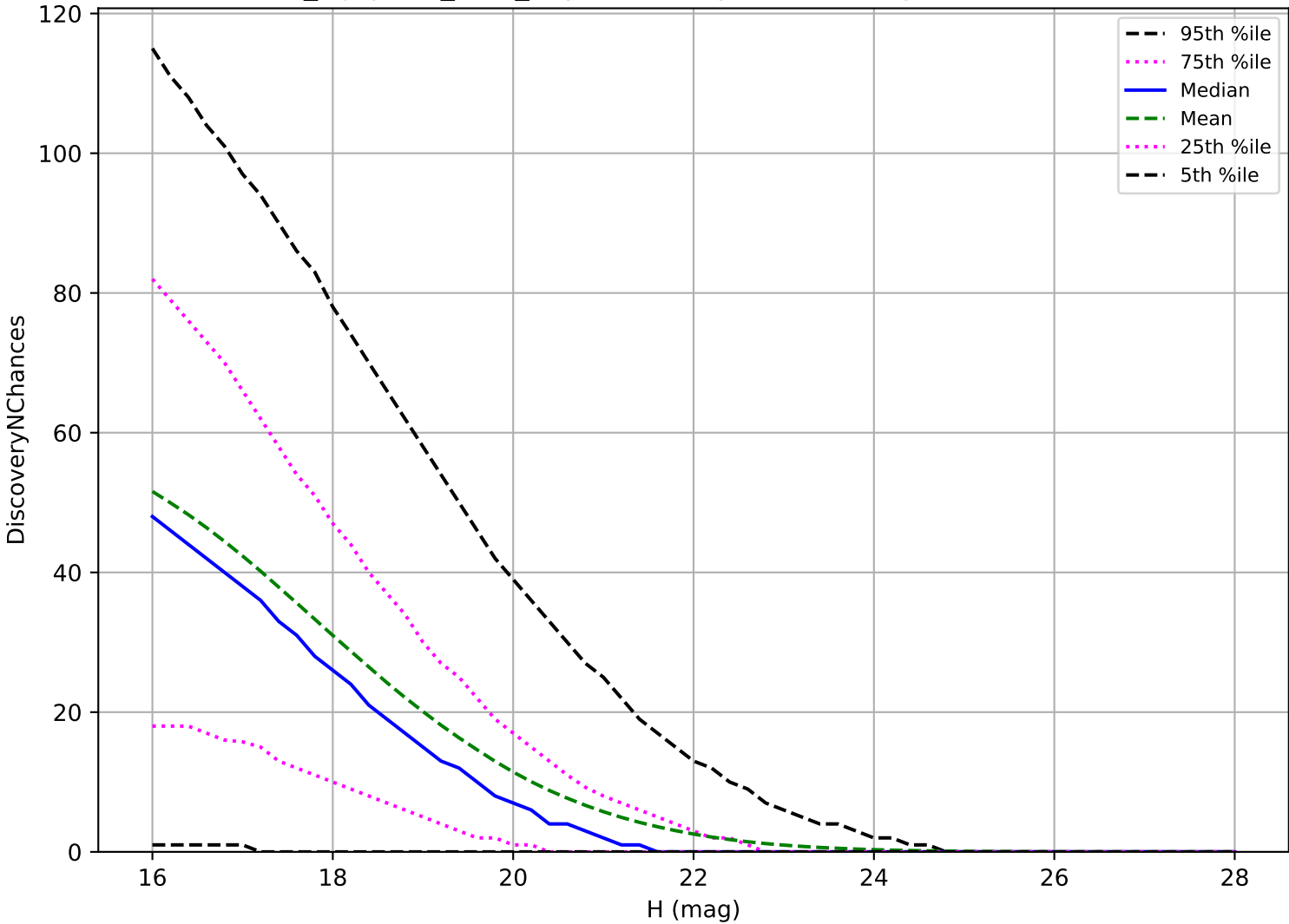
noroll_mjdp365_v3.4_10yrs: PHA 3 pairs in 15 nights detection loss
