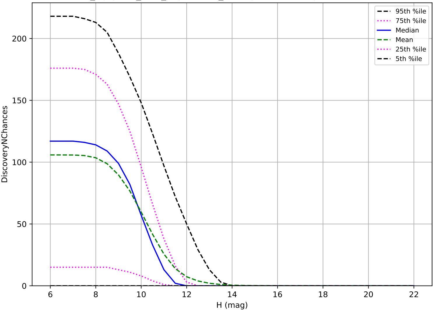
noroll_mjdp365_v3.4_10yrs: OCC_r20 3 pairs in 15 nights detection loss
