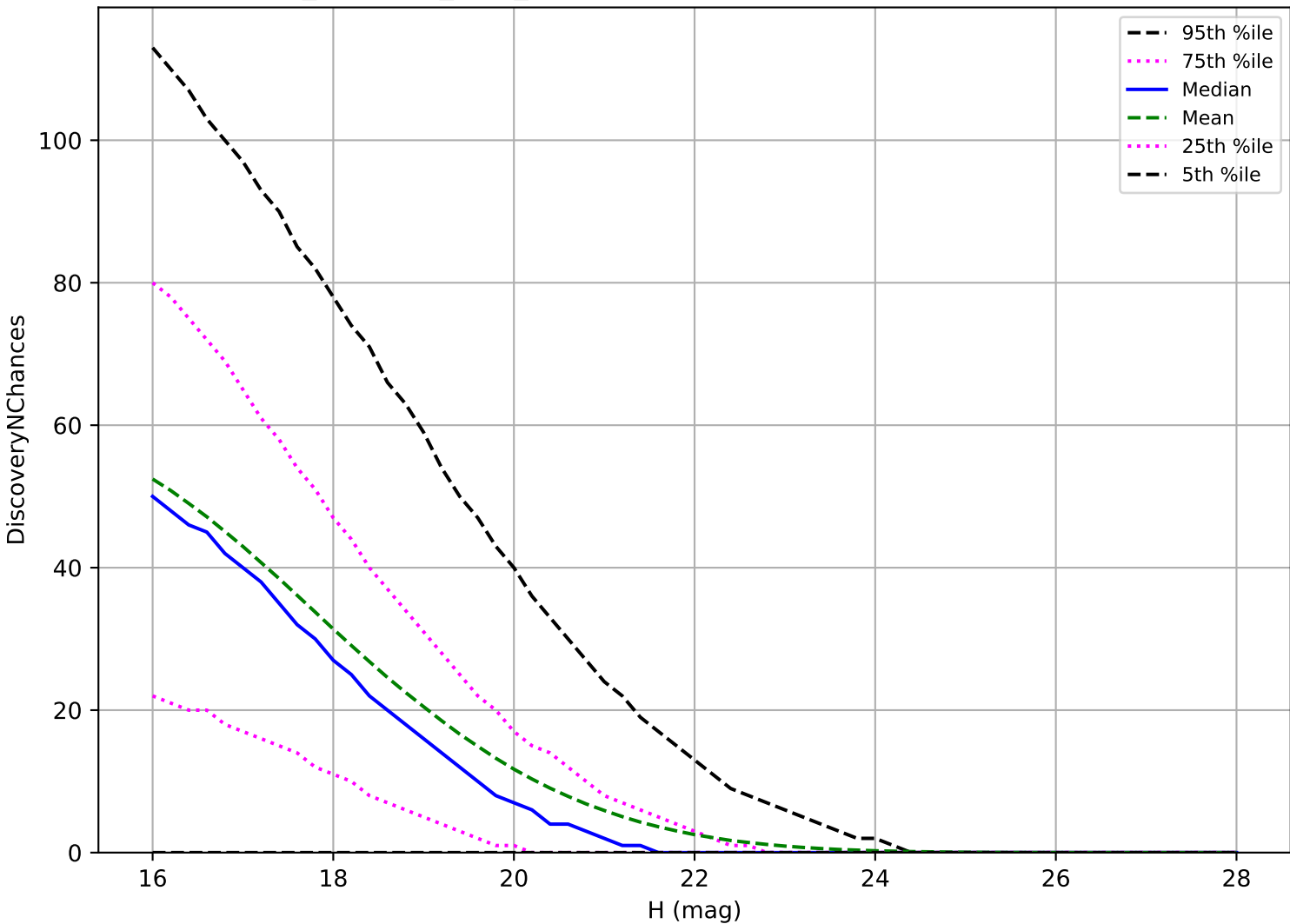
noroll_mjdp365_v3.4_10yrs: NEO 3 pairs in 15 nights detection loss
