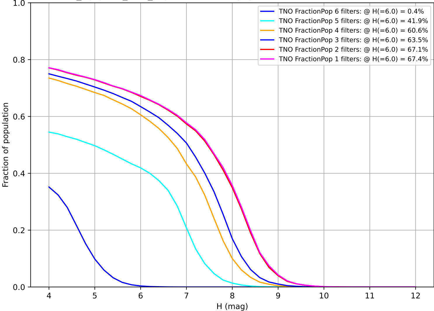
noroll_mjdp365_v3.4_10yrs: Fraction of population with colors in X filters TNO
