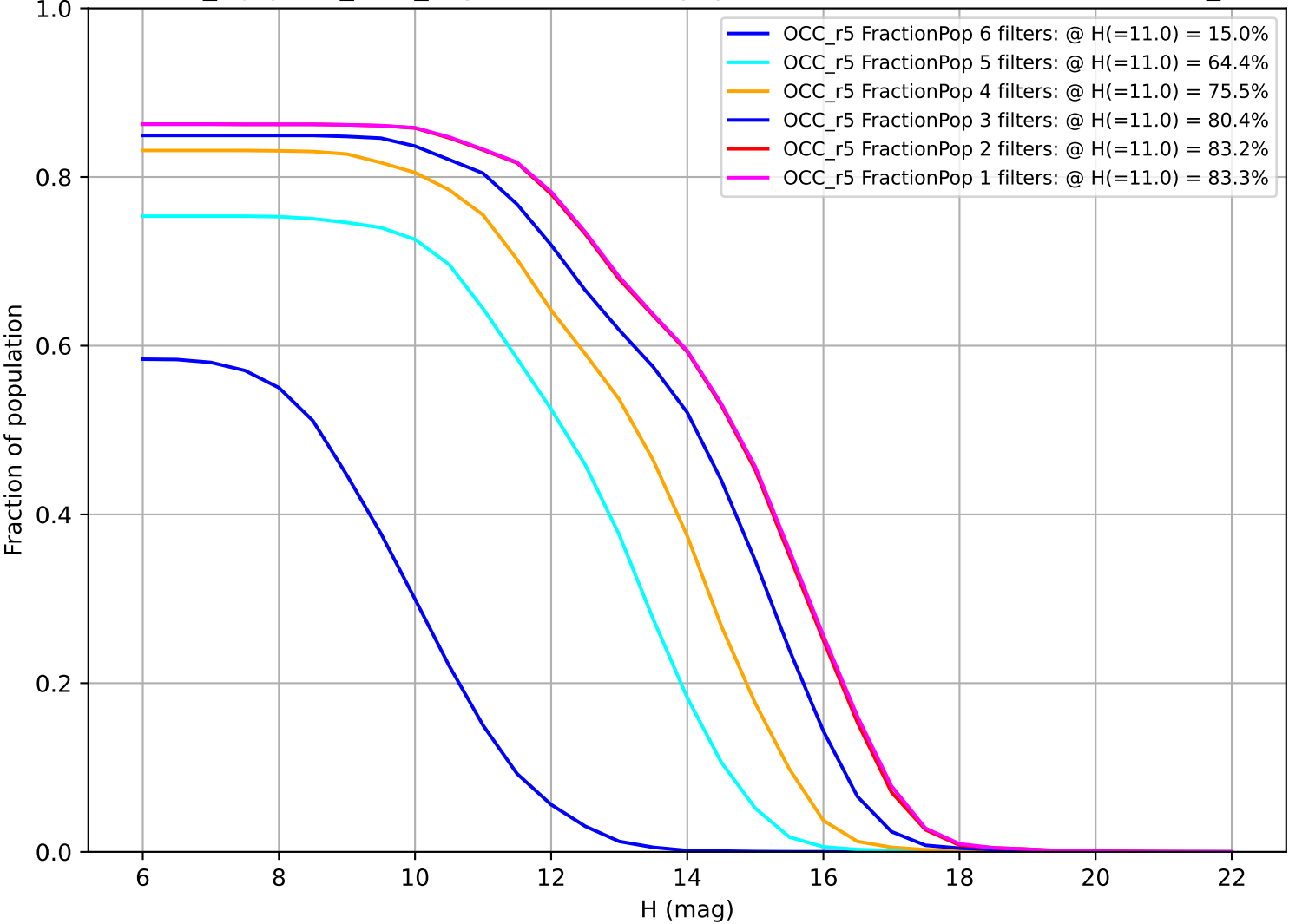
noroll_mjdp365_v3.4_10yrs: Fraction of population with colors in X filters OCC_r5
