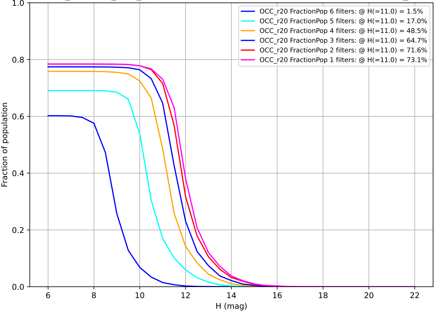
noroll_mjdp365_v3.4_10yrs: Fraction of population with colors in X filters OCC_r20
