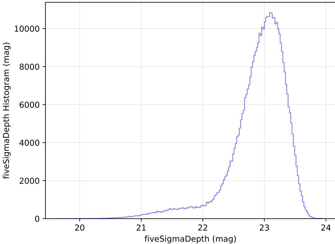
noroll_mjdp365_v3.4_10yrs z: fiveSigmaDepth Histogram
