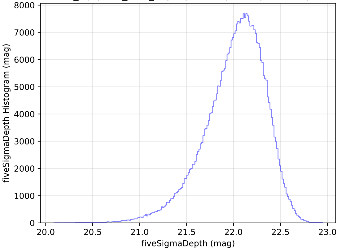
noroll_mjdp365_v3.4_10yrs y: fiveSigmaDepth Histogram
