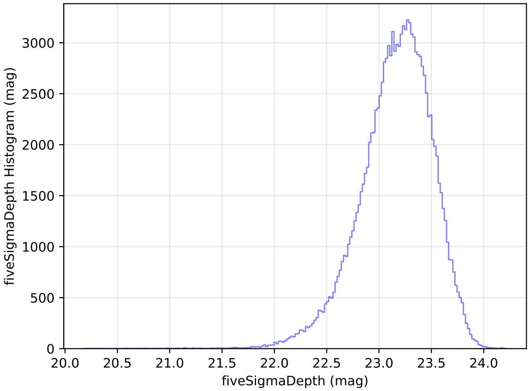
noroll_mjdp365_v3.4_10yrs u: fiveSigmaDepth Histogram
