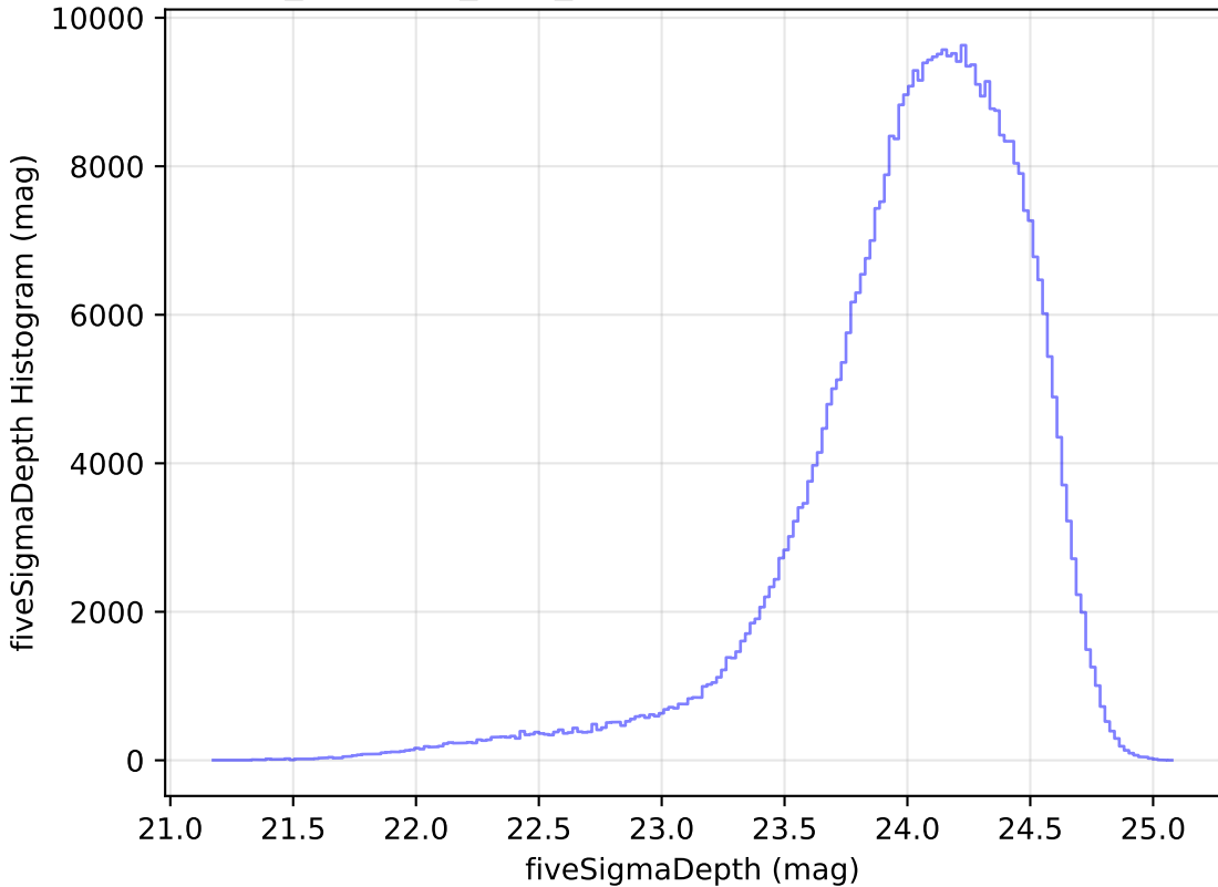
noroll_mjdp365_v3.4_10yrs r: fiveSigmaDepth Histogram
