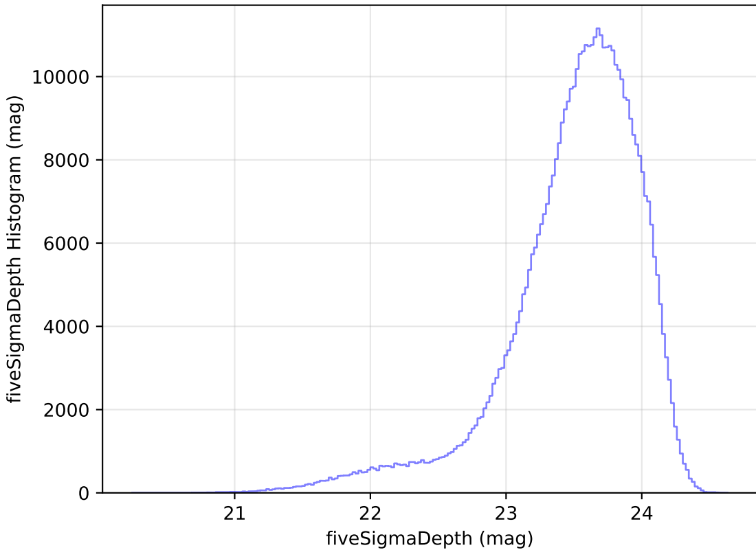
noroll_mjdp365_v3.4_10yrs i: fiveSigmaDepth Histogram
