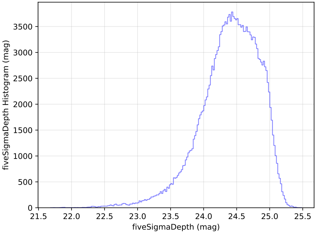
noroll_mjdp365_v3.4_10yrs g: fiveSigmaDepth Histogram
