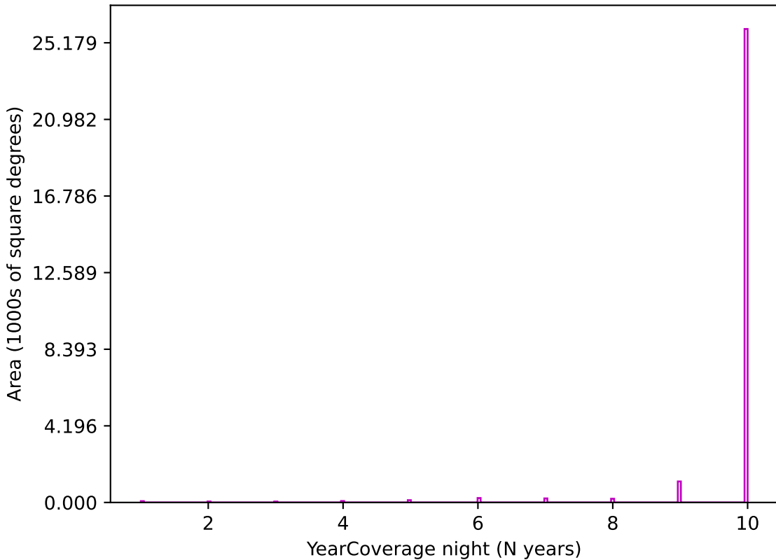
noroll_mjdp365_v3.4_10yrs z band: YearCoverage night
