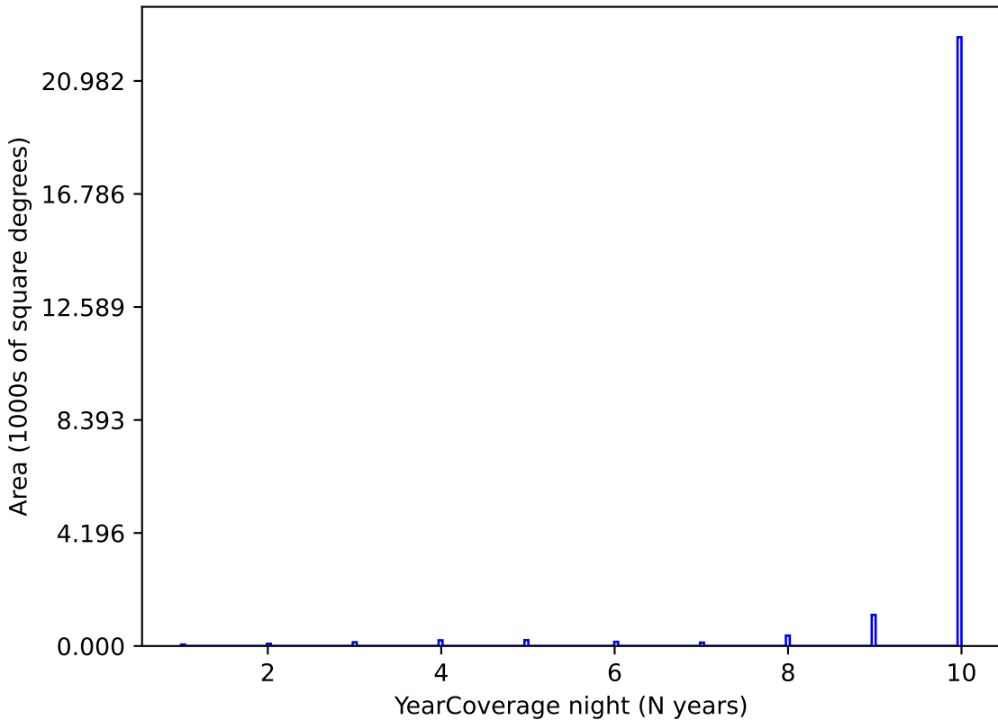
noroll_mjdp365_v3.4_10yrs y band: YearCoverage night
