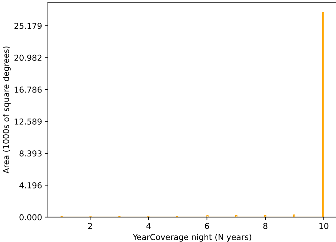
noroll_mjdp365_v3.4_10yrs r band: YearCoverage night
