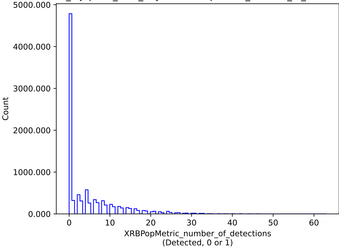
noroll_mjdp365_v3.4_10yrs : XRBPoMetric_number_of_detections
