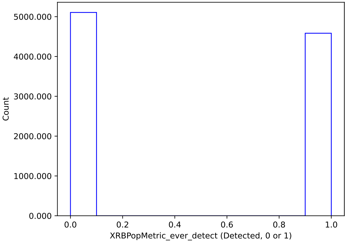
noroll_mjdp365_v3.4_10yrs : XRBPopMetric_ever_detect
