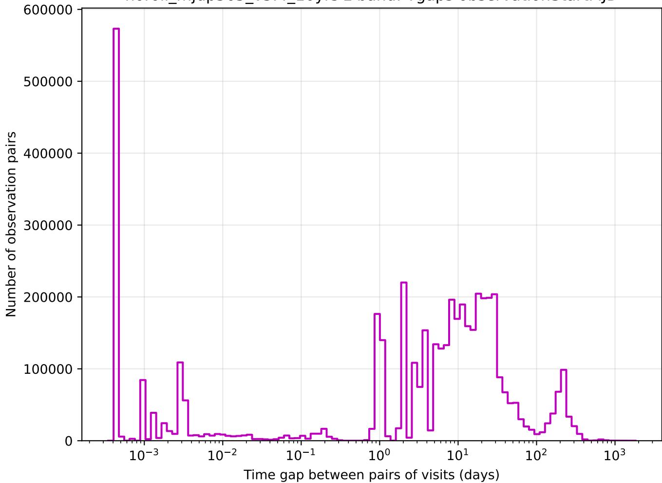
noroll_mjdp365_v3.4_10yrs z band: Tgaps observationStartMJD
