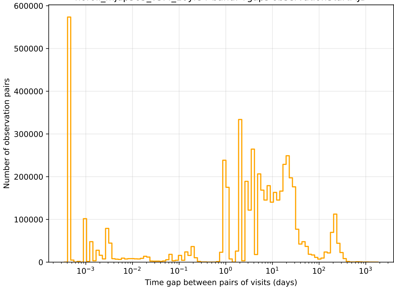
noroll_mjdp365_v3.4_10yrs r band: Tgaps observationStartMJD
