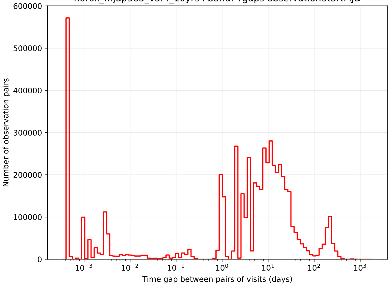
noroll_mjdp365_v3.4_10yrs i band: Tgaps observationStartMJD
