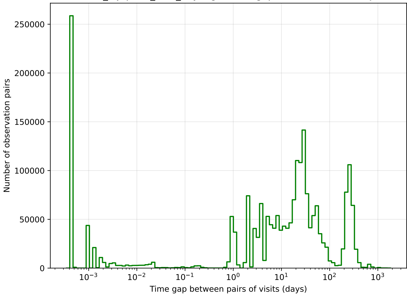
noroll_mjdp365_v3.4_10yrs g band: Tgaps observationStartMJD
