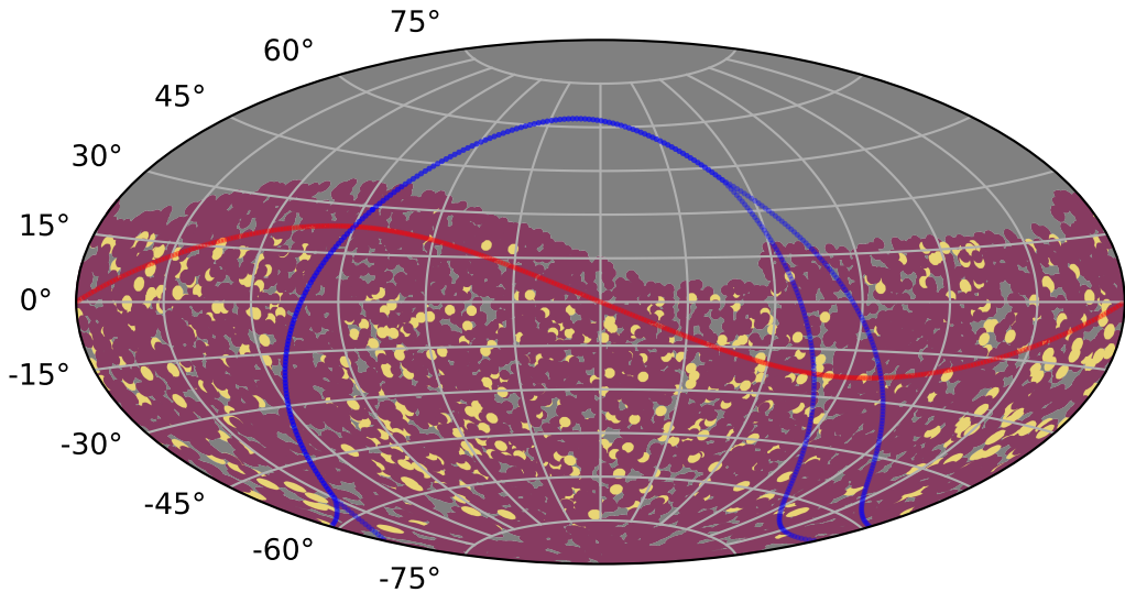
noroll_mjdp365_v3.4_10yrs : TDEsPopMetric_some_color
