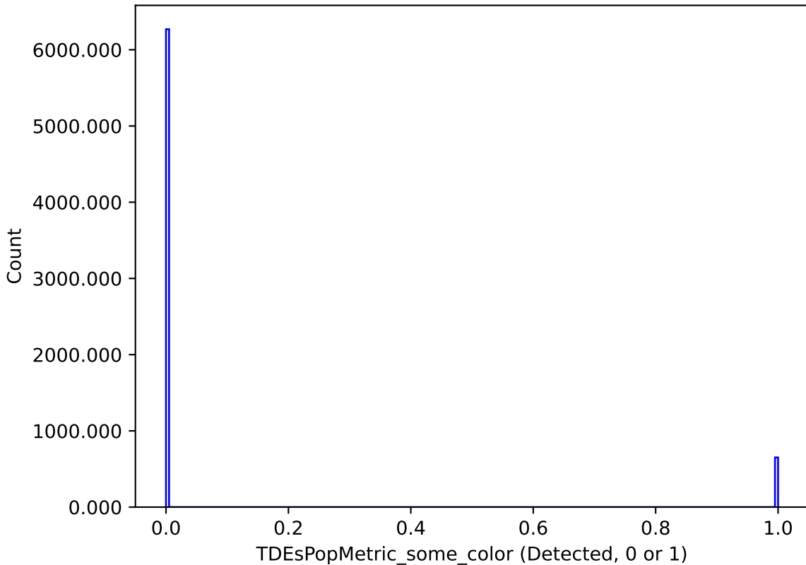
noroll_mjdp365_v3.4_10yrs : TDEsPopMetric_some_color
