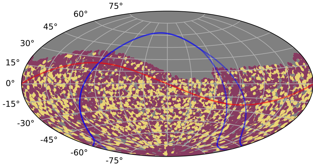
noroll_mjdp365_v3.4_10yrs : TDEsPopMetric_prepeak
