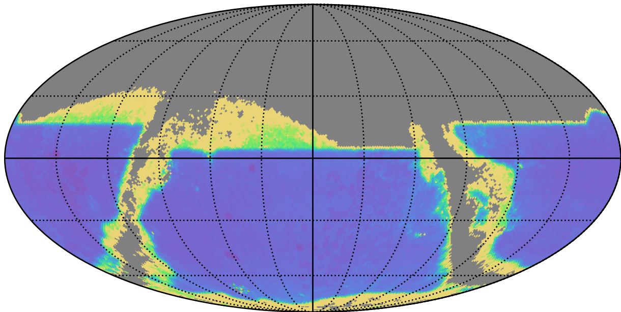
noroll_mjdp365_v3.4_10yrs : TDC_precision
