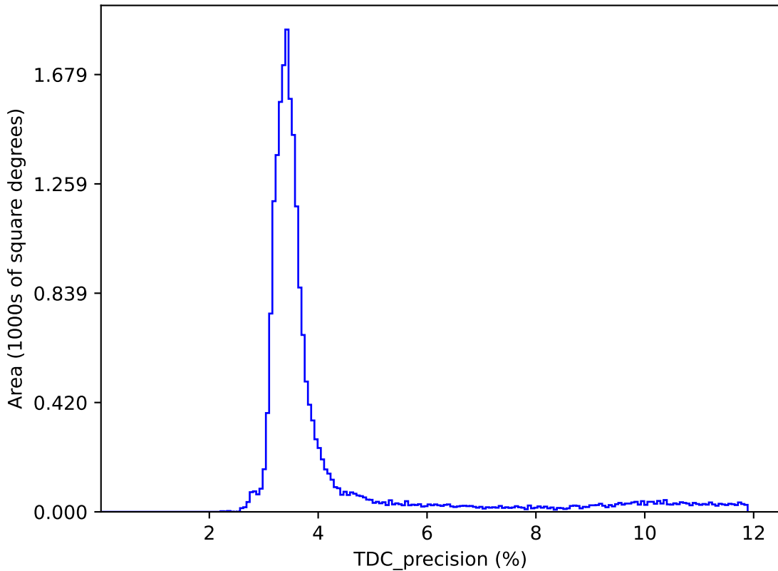
noroll_mjdp365_v3.4_10yrs : TDC_precision
