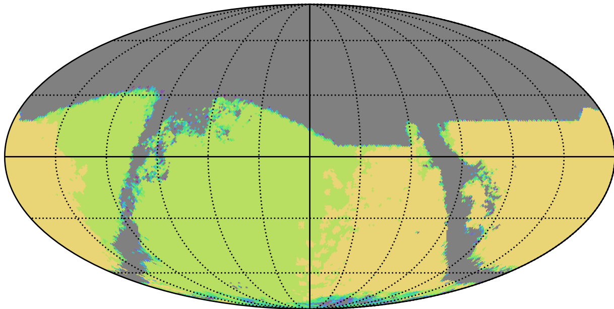
noroll_mjdp365_v3.4_10yrs : TDC_campaign
