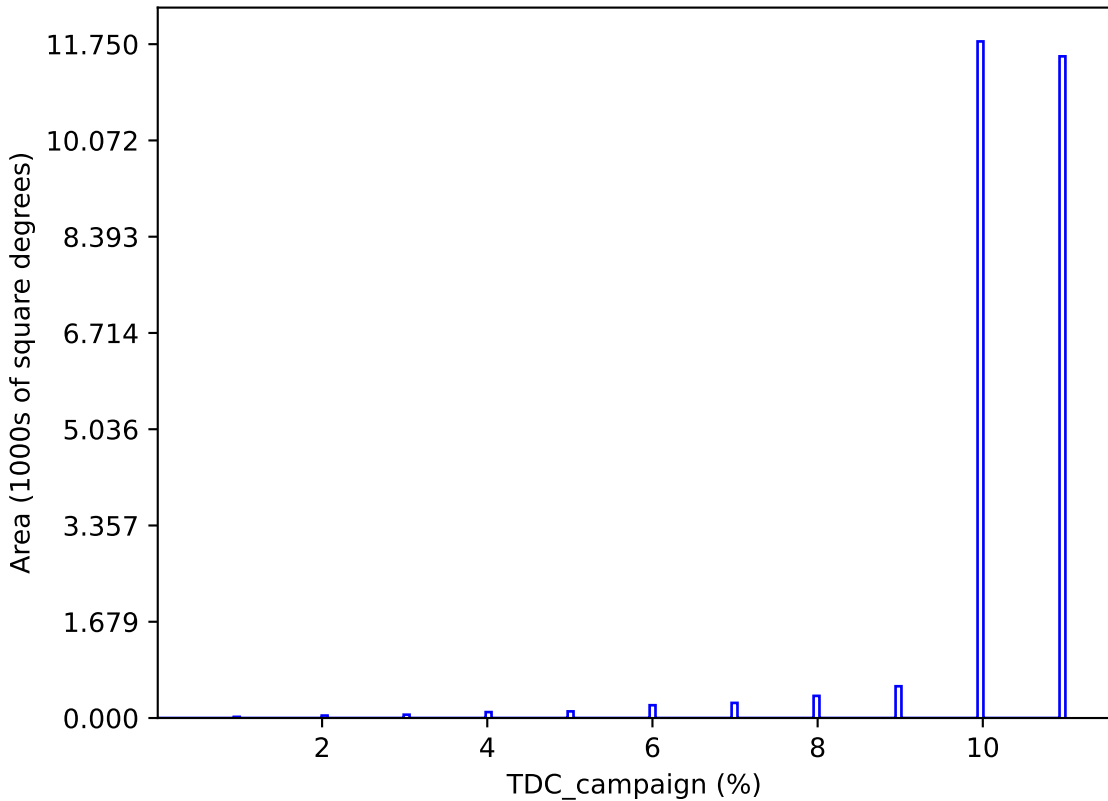
noroll_mjdp365_v3.4_10yrs : TDC_campaign
