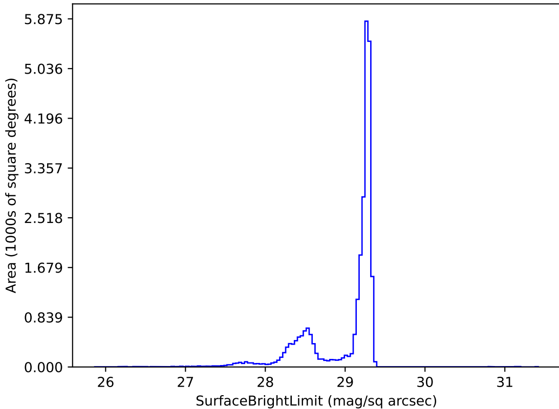
noroll_mjdp365_v3.4_10yrs z: SurfaceBrightLimit
