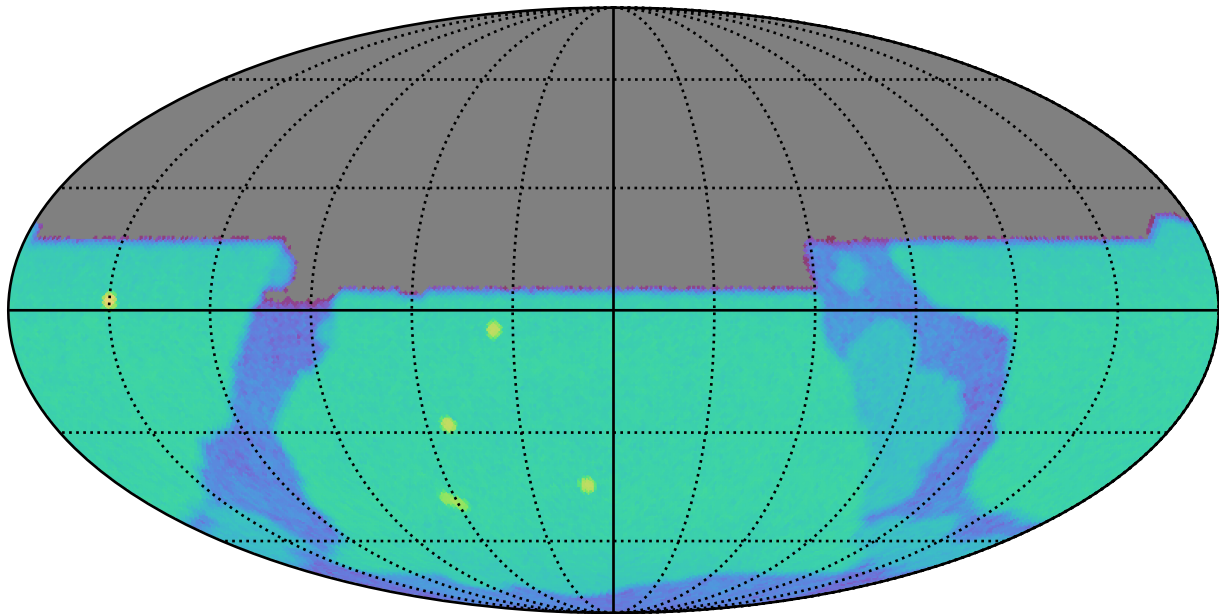
noroll_mjdp365_v3.4_10yrs u: SurfaceBrightLimit
