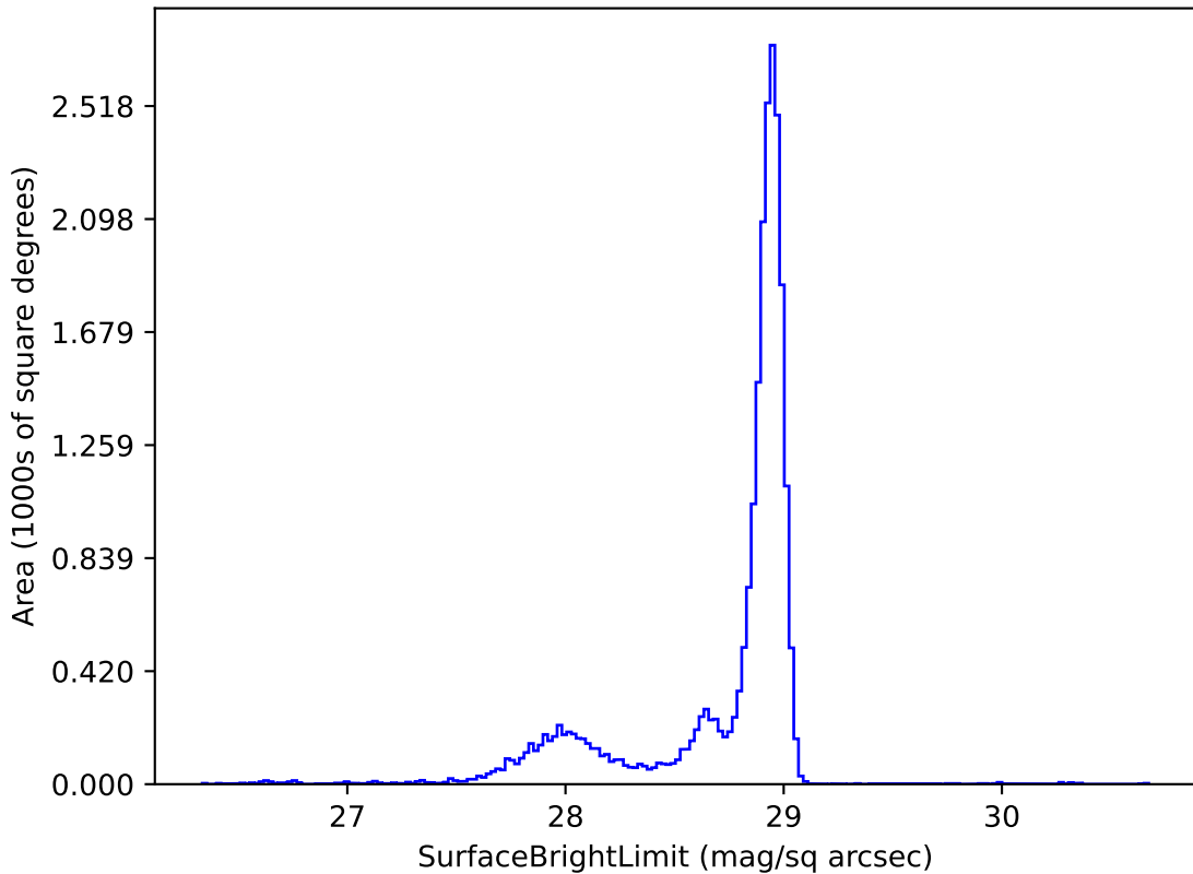
noroll_mjdp365_v3.4_10yrs u: SurfaceBrightLimit
